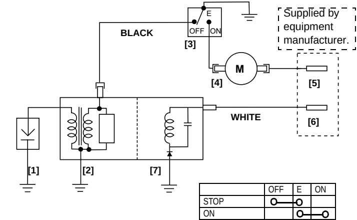
ELECTRIC STARTER (with flywheel brake)
